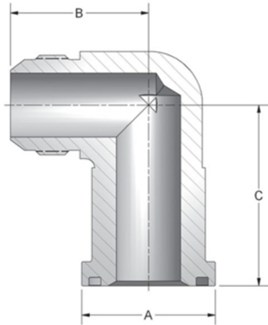
CD61/CD62 90 Degree Elbow JIC Thread Split Flange Adapters
