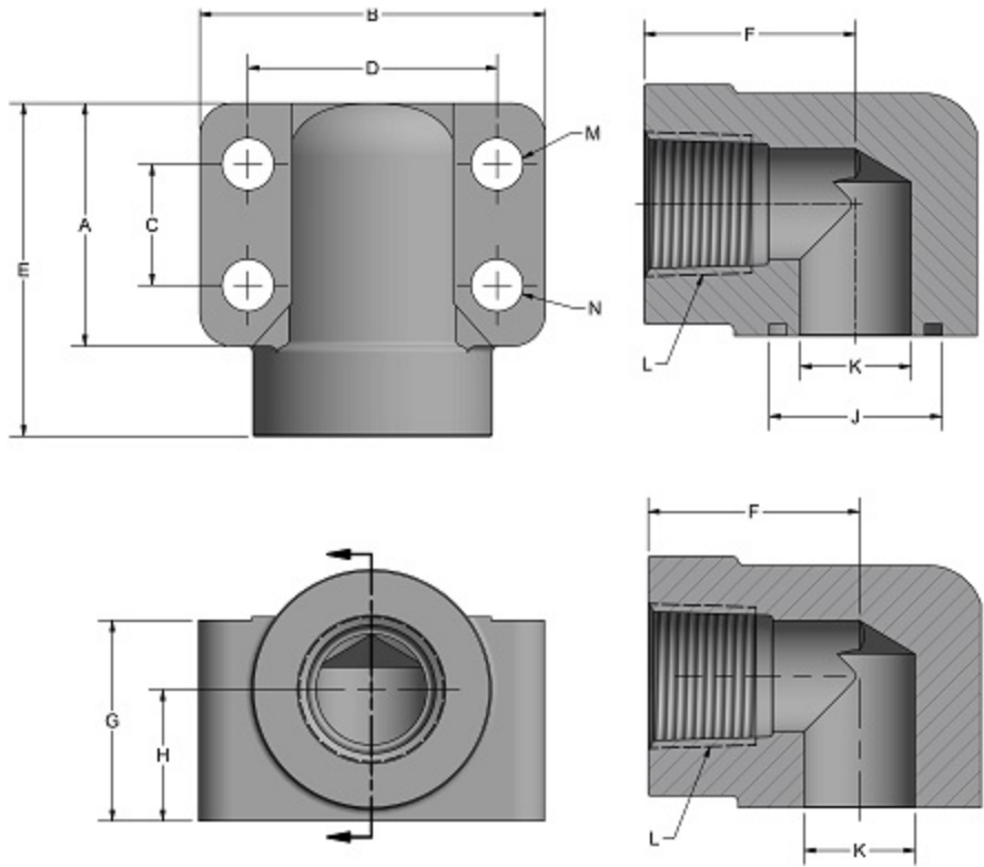
CD61/CD62 Elbow NPTF & SAE Thread 4-Bolt Flanges
