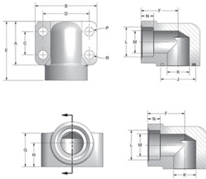
CD61 Elbow Socket Weld Pipe 4-Bolt Flanges
