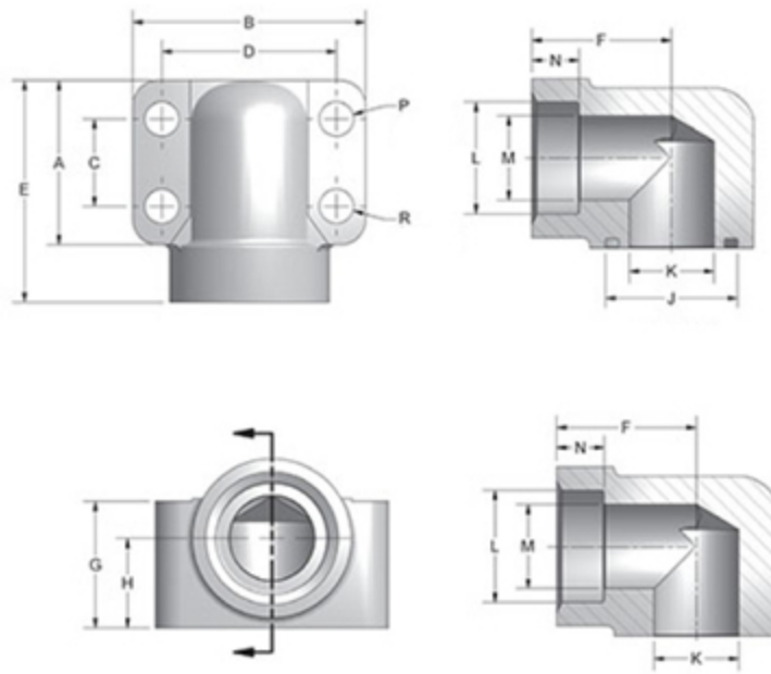
CD61 Elbow Socket Weld Pipe 4-Bolt Flanges
