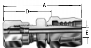
SAE male flareless with nut and ferrule 190609-
