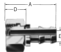
Metric universal female swivel 60° DIN 7631/7647 07.006–/07.001–/07.114–
