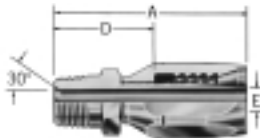
Male pipe 190934-/FC7640-
