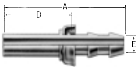
Compression type 4750-
