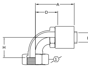
ORS® Swivel 90° elbow (short) FJ9612/FJ9898
