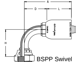
BSPP Swivel 90° Elbow
