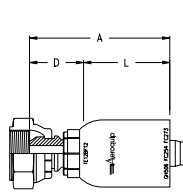
BSPP Swivel Straight
