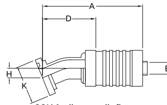
22½° elbow split flange FC5372 Code 62
