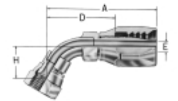
SAE 37° (JIC) swivel 60° elbow FC5984-/FJ9024-
