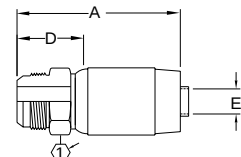
SAE 37° (JIC) male flare FJ9917
