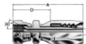
30° swivel-metric threads special Komatsu FJ7201-
