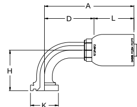
Code 62 90° Elbow Split Flange
