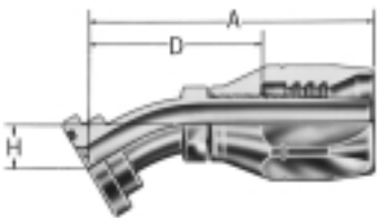
22½° split flange FC9634-/FC7714- Code 61 SAE J518 FC7983-/FC5974- Code 62 SAE J518
