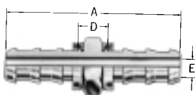
Hose mender 4772-
