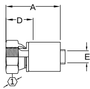
SAE 37° (JIC) swivel FJ9587
