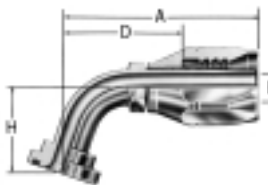
60° split flange
