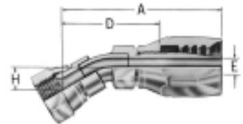
SAE 37° (JIC) swivel 30° elbow FC5980-/FC5981-
