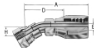
SAE 37° (JIC) swivel 22 1/2° elbow FC5978-/FC5979-
