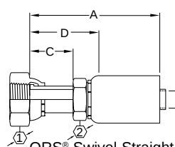
ORS® Swivel Straight FJ9480
