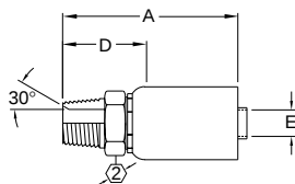
Swage male pipe fitting FJ9372/FJ5020
