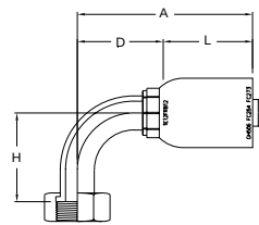
ORS® Swivel 90° Elbow
