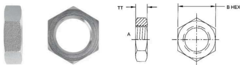
PART NO. TUBE O.D. A THREAD B HEX TT WIDTH
