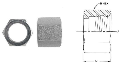
PART NO. TUBE O.D. A THREAD B HEX Q WIDTH
