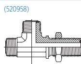
FS2704* MFS-MFS-MFS Bulkhead Tee
