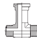
FS1805 MFS-MFS- Flange Tee Code 62
