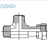
FS6602 MFS-FFSS-MFS Run Tee
