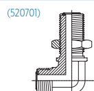
FS2701* MFS-MFS Bulkhead 90°
