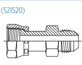
FS6504 FFSS-MJ Straight
