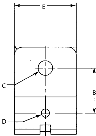
Figure 1 Bracket Top
