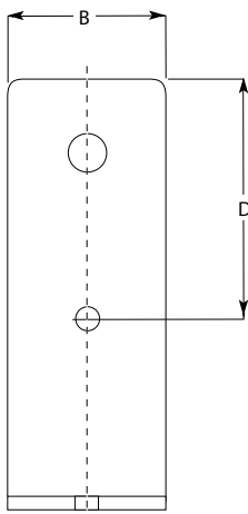
Figure 3 Base Bracket
