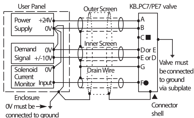
Figure 1. Wiring connections for valves with integral amplifier
