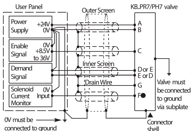
Figure 2. Wiring connections for valves with "Enable" feature
