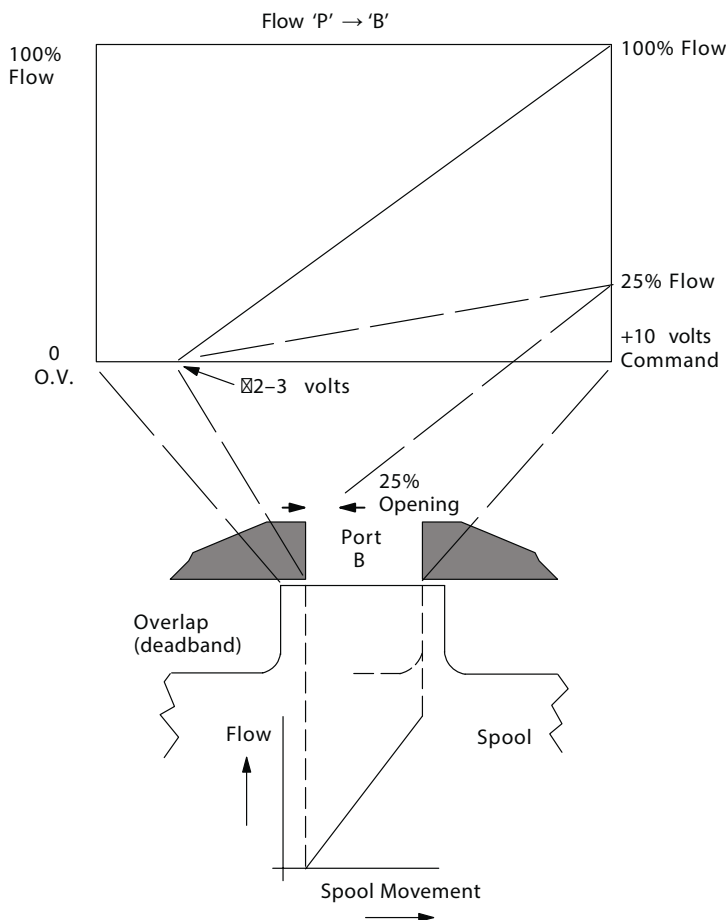
Figure 6. Gain Control
