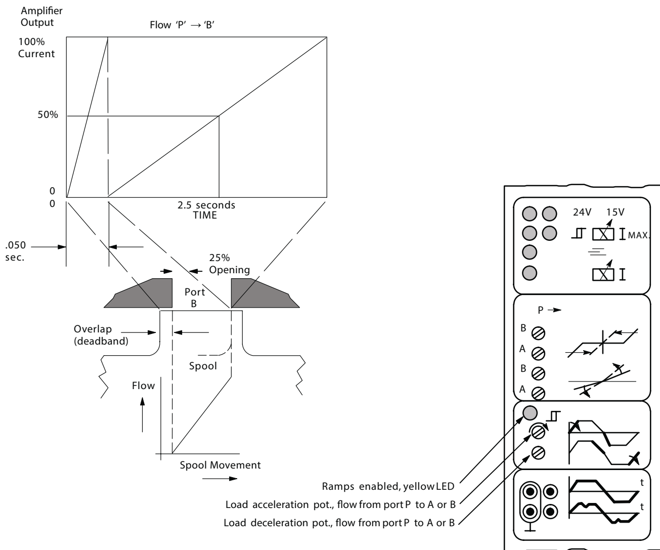
Figure 12. Ramp Function
