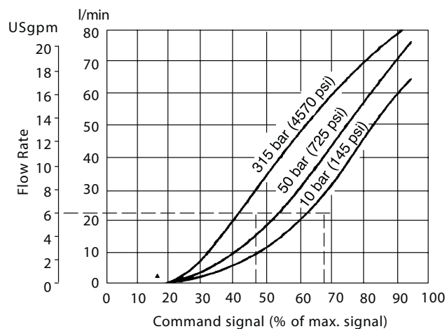
Figure 4. Pressure Drop
