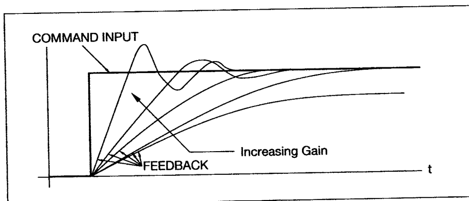
Figure 3. Increasing Proportional Gain.
