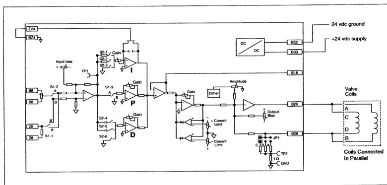
Figure 1. Servovalve amplifier set-up connections
