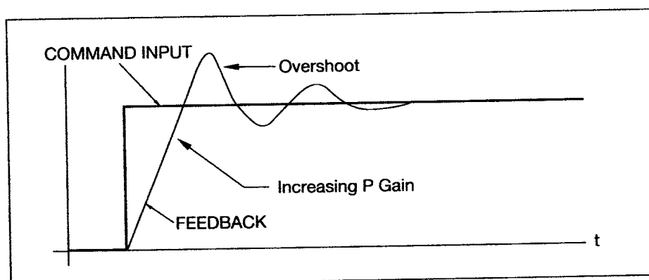
Figure 5. Moderate overshoot.
