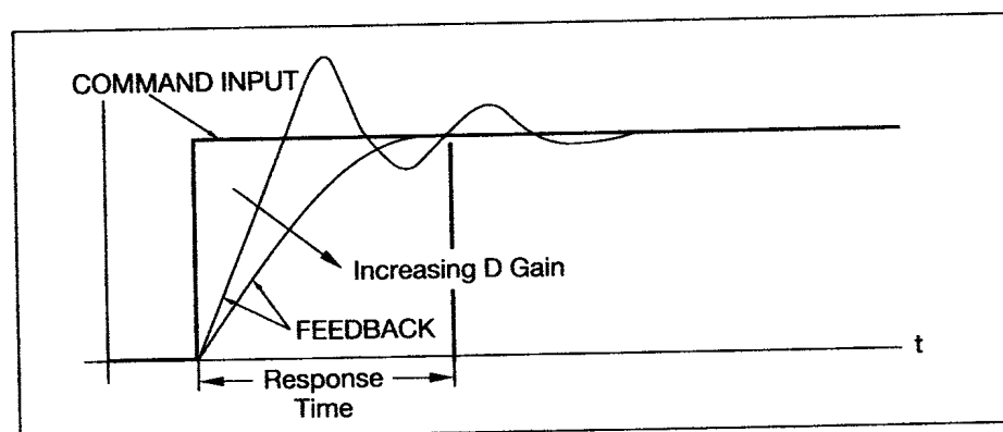
Figure 6. Eliminated overshoot by adding Derivative Gain.
