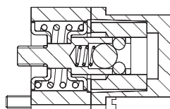
Detent spool out
