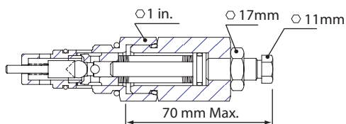
External adjust anti-cavitation relief
