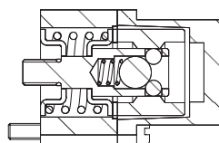
Detent in and out
