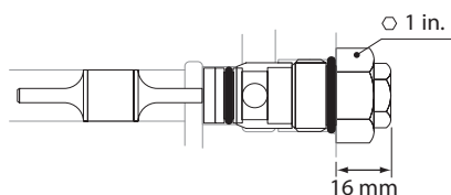
Pilot check valve
