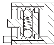
3-position detent
