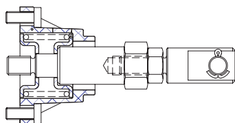
Spring center with male extension
