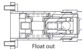
Spring center with 4th position detent float
