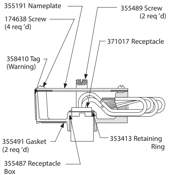
Receptacle Kit 942067
