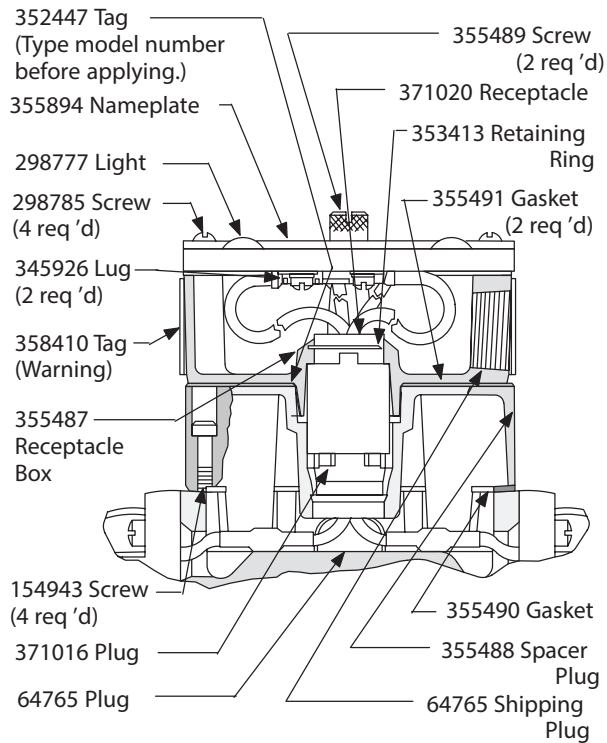
Plug & Receptacle with Double Indicator Light Kit 942066 (100 thru 127V AC) 941182 (192 thru 233V AC)
