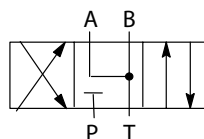
Type 6N Detent A&B to Tank, P Blocked P/N 681615
