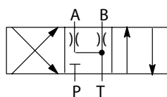
Type 33B/C Closed Center, (Bleed A & B) P/N 617123
