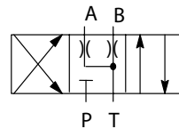
Type 33 Controlled Leakage from A & B to Tank, P Blocked P/N 399897
