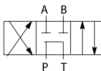
Type 4 Tandem with Closed Center Crossover P/N 281926
