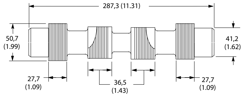
Type 33 Controlled Leakage from A & B to Tank, P Blocked P/N 364042
