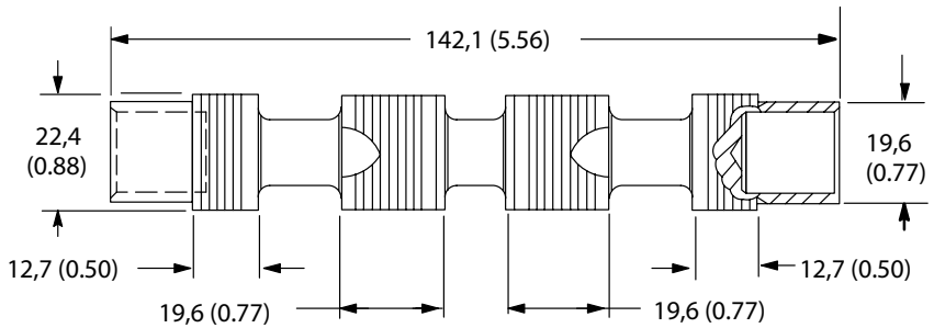
Type 33 Controlled Leakage from A & B to Tank, P Blocked P/N 399897
