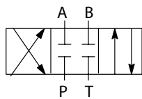
Type 2 Closed Center P/N 363496
