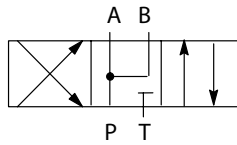
Type 7B Open Center, P to A & B, Tank Blocked P/N 617125
