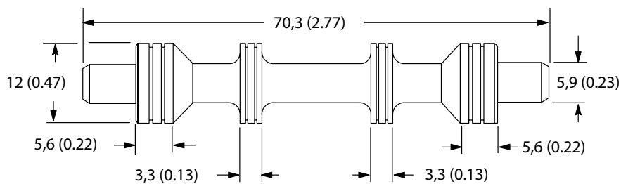
Type 0 Spring Centered, Spring Offset Open Center P/N 694435
