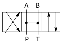
Type 0 Spring Centered, Spring Offset Open Center P/N 694435
