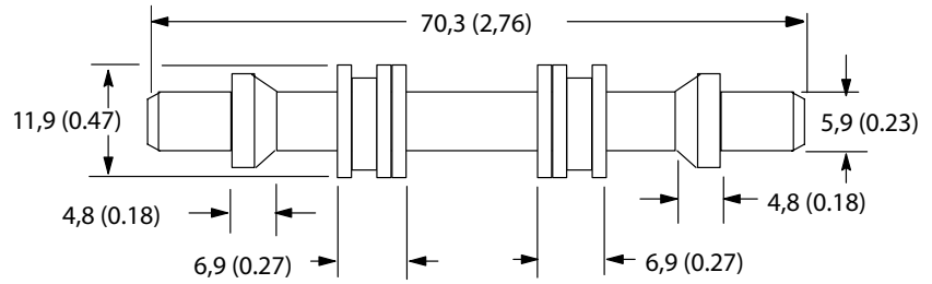
Type 7B Open Center, P to A & B, Tank Blocked P/N 617125
