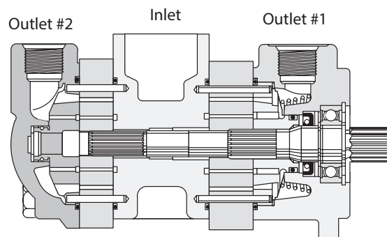
Assembly View
