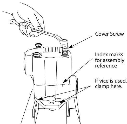
Figure 10. Beginning disassembly
