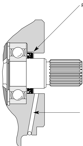
Figure 6a. Single Shaft Seal Models
