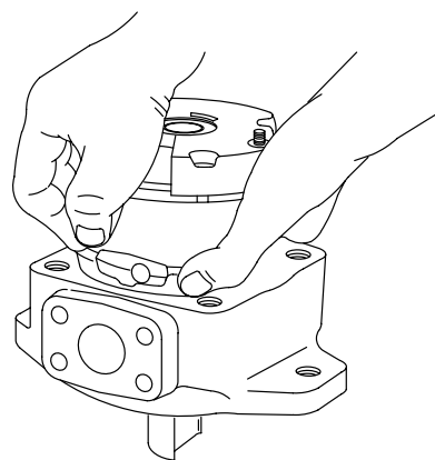
Figure 11. Cartridge removal
