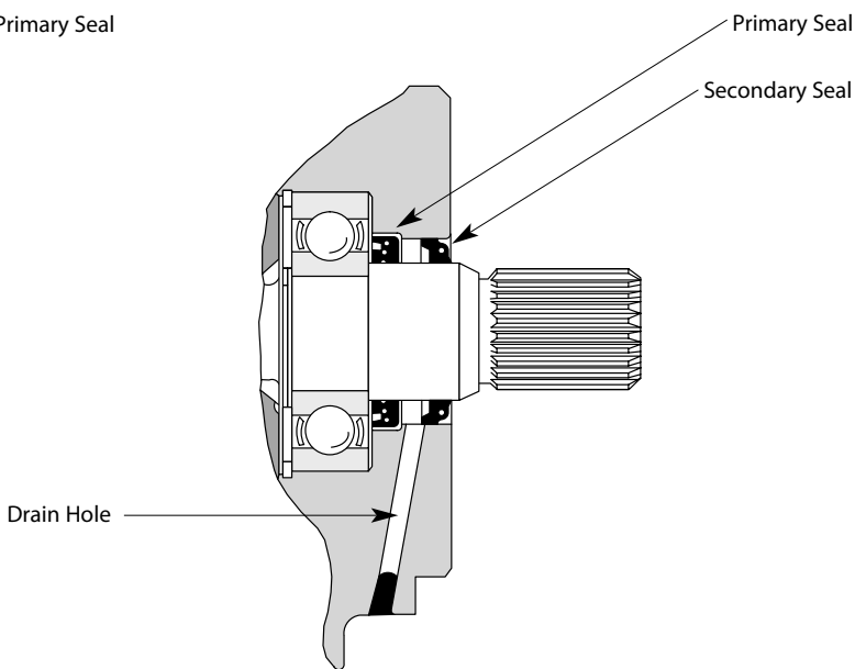
Figure 6b. Double Shaft Seal Models
