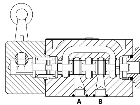
DG20V—3—*C—60 Sectional View Spring Centered
