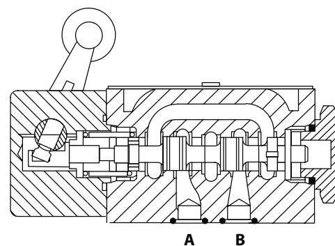
DG20V—3—*A—60 Sectional View Spring Offset, Offset to Cam Position # 3
