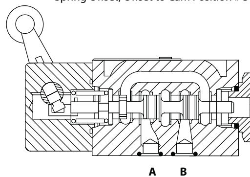
DG20V—3—*A—60 Sectional View Spring Offset, Offset to Cam Position # 3
