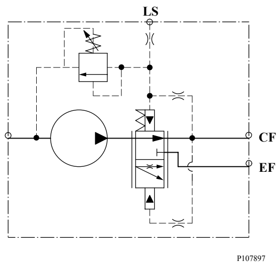
D Series Pump with Load Sensing Schematic
