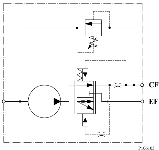
D Series Pump with Load Sensing Schematic
