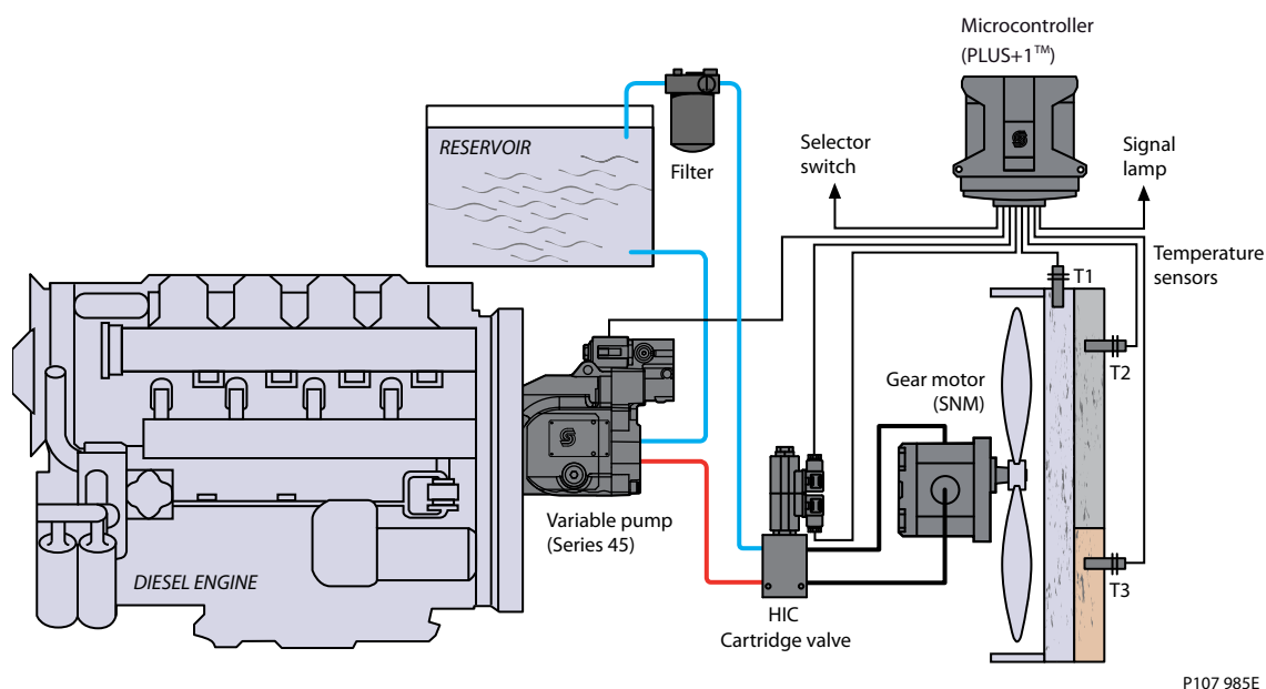
Variable Pump with HIC Cartridge Valve
