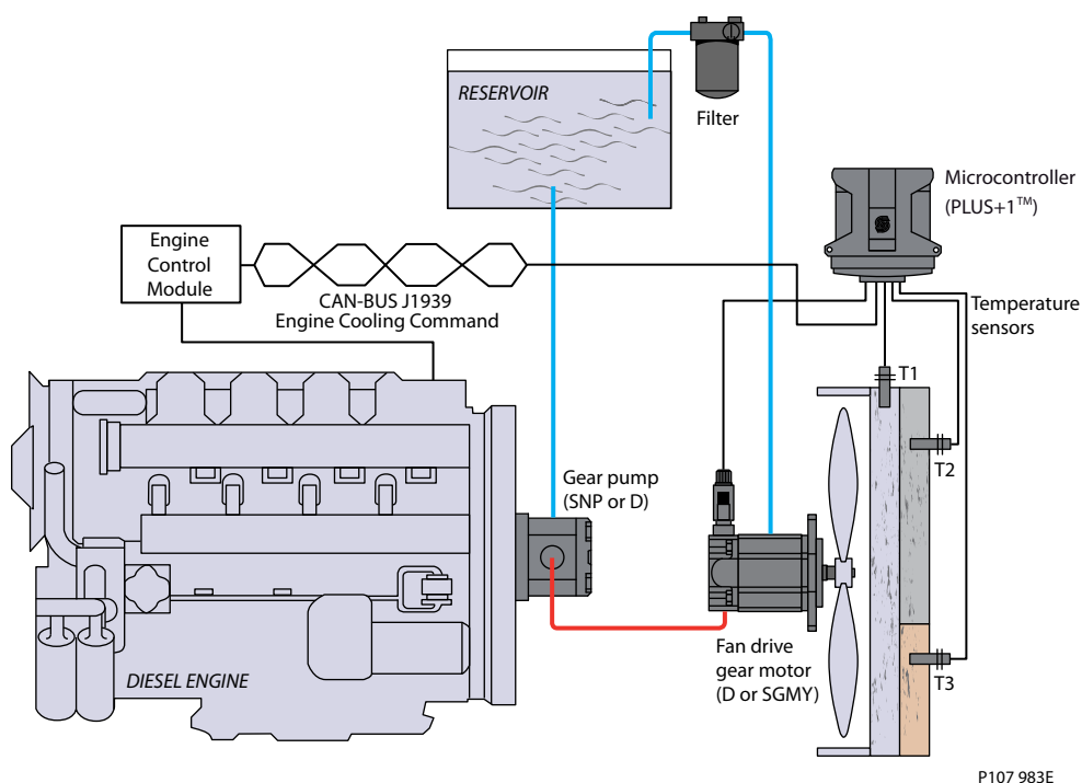
PLUS+1™ System Illustration
