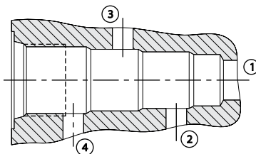
Cavity 4 way
