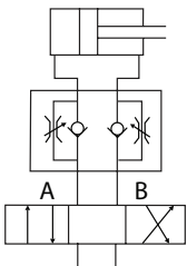
Meter-out control...Y
