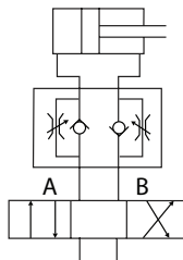
A Meter-in control B Meter-out control: XY
