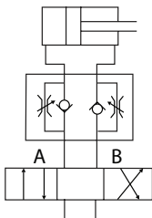
A Meter-out control B Meter-in control: YX
