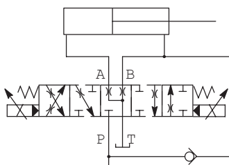
Spool type 133C with typical regenerative circuit
