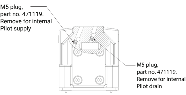
KBDG5V-7 Models Viewed from port A end of main stage
