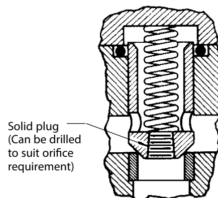
Construction of "S12" Cracking Pressures Model
