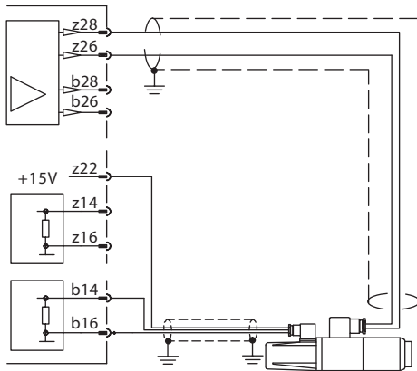
Amplifier models: 541, 581
