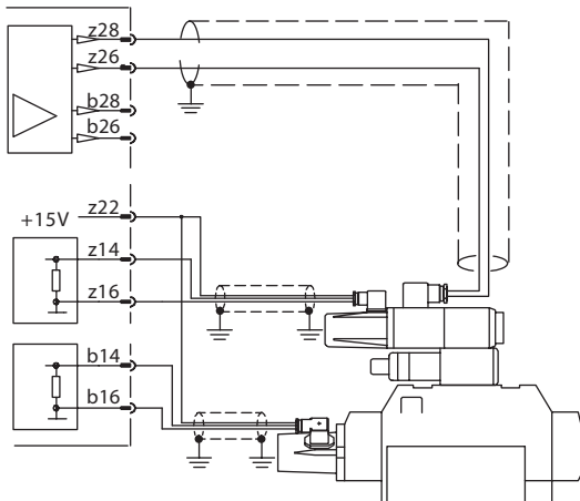
Amplifier models: 541, 581
