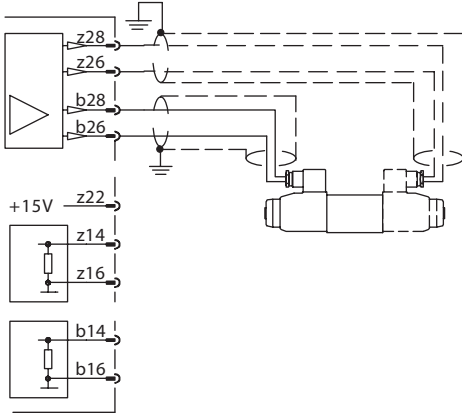
Amplifier model: 553
