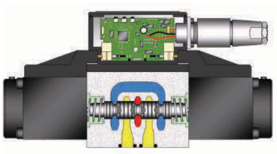
KBDG4V-5-PE, 1 * Series
