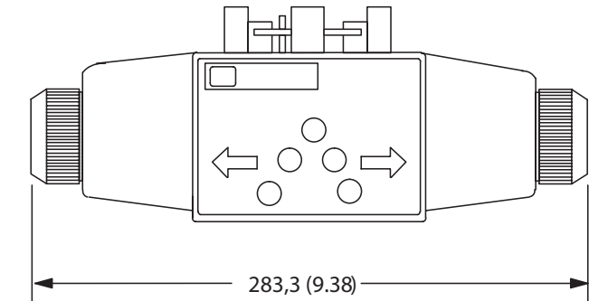
Single Solenoid Valve (PA3)
