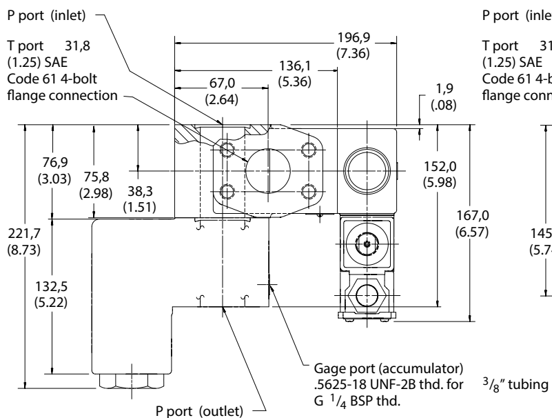
"C" Models Right Angle Check
