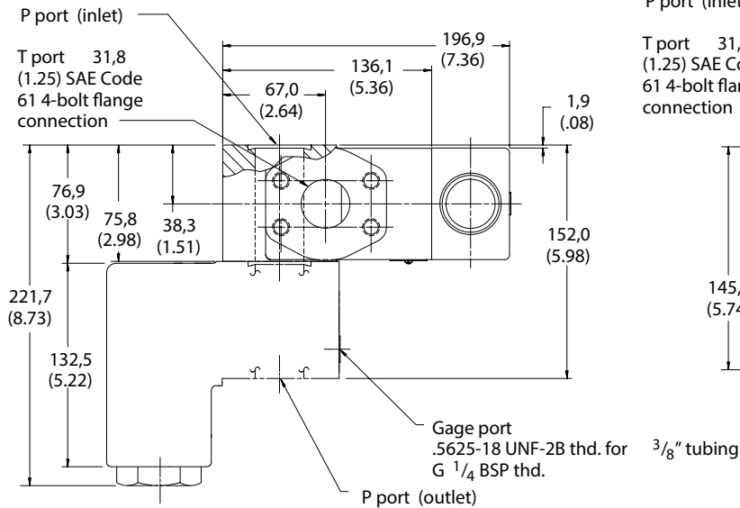
"C" Models Right Angle Check
