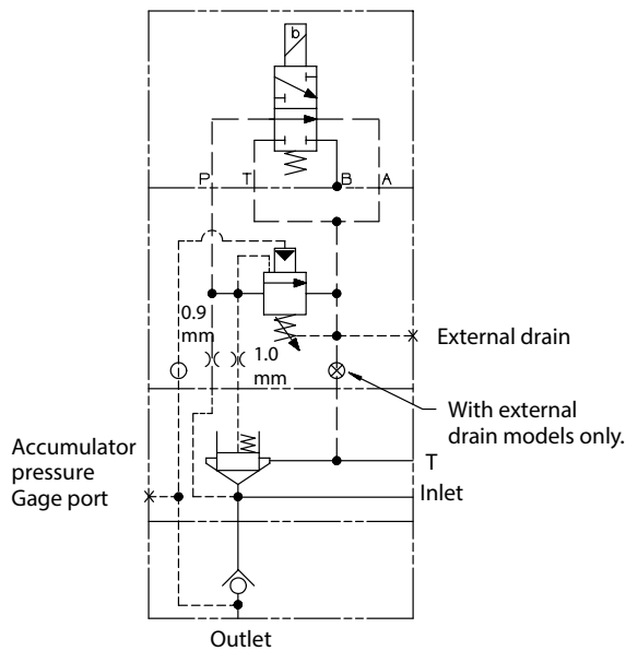
UPF2S-C*-10/12-*-20 with check valve and vent
