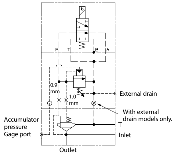
UPF2S-10/12-(P)*-20 with vent and without check valve
