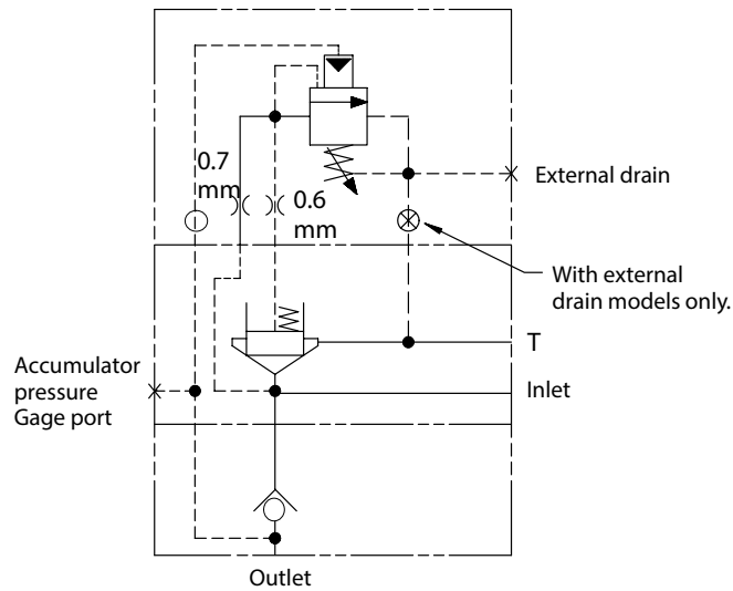
UPF15-C*-06/08-*-20 with check valve
