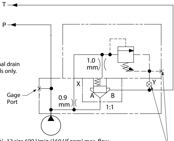
CPF1S-10/12-P-*-20 without remote control
