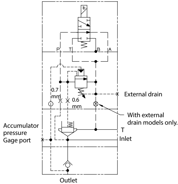
UPF2S-C*-06/08-*-20 with check valve and vent
