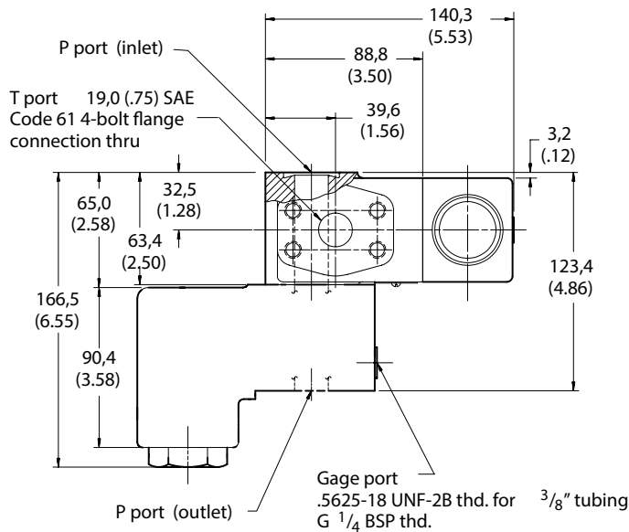
"C" Models Right Angle Check
