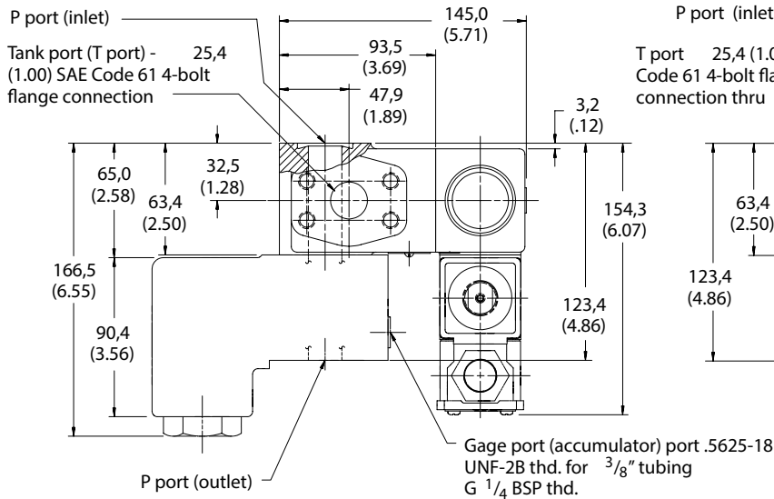
"C" Models Right Angle Check
