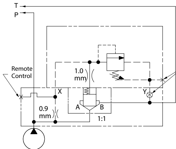
CPF1S-10/12-*-20 with remote control
