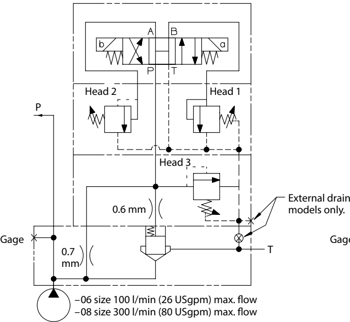
CPF3S-06/08-*-20
