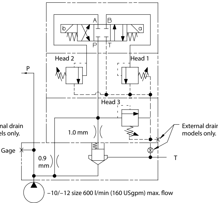
CPF4S-10/12-*-20 CPF4V-12-*-20
