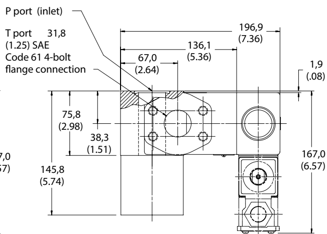
"CL" Models In-line Check
