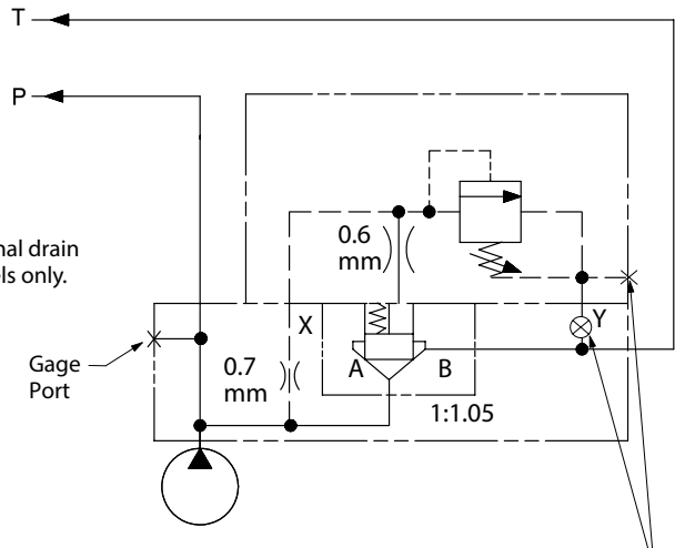
CPF1S-06/08-P-*-20 without remote control
