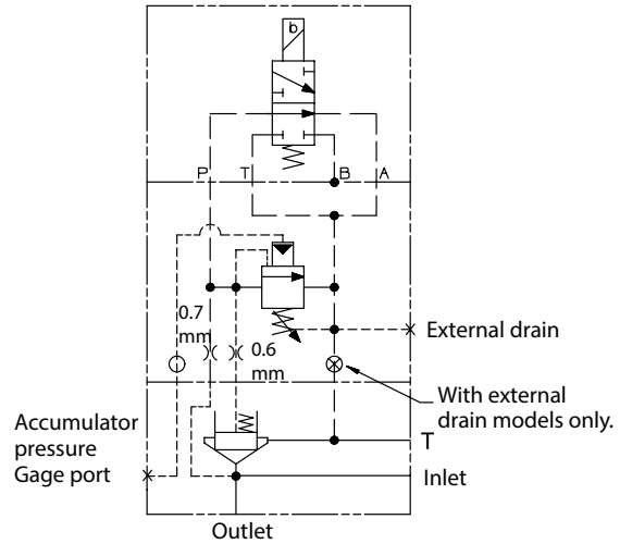
UPF2S-06/08-(P)*-20 with vent and without check valve
