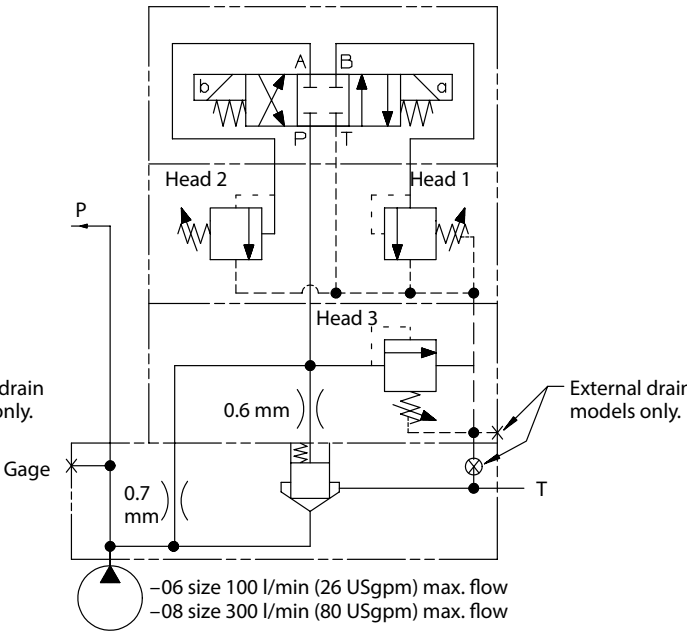
CPF4S-06/08-*-20
