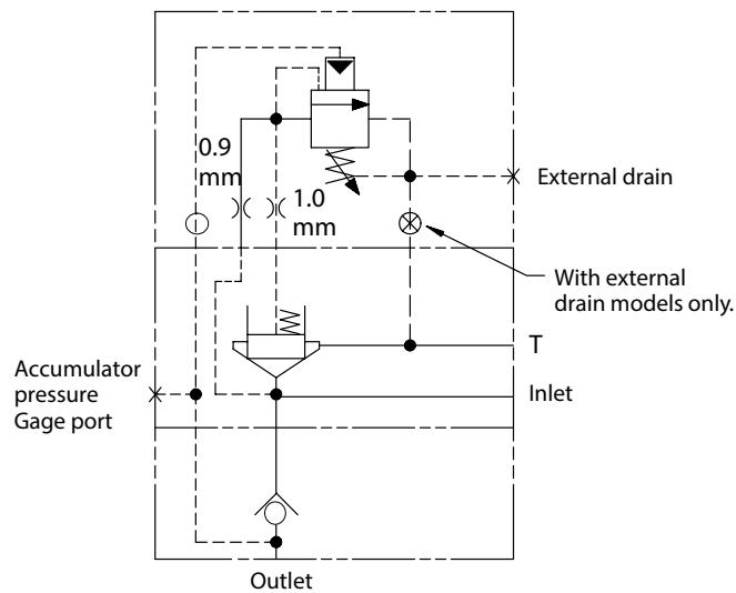
UPF15-C*-10/12-*-20 with check valve
