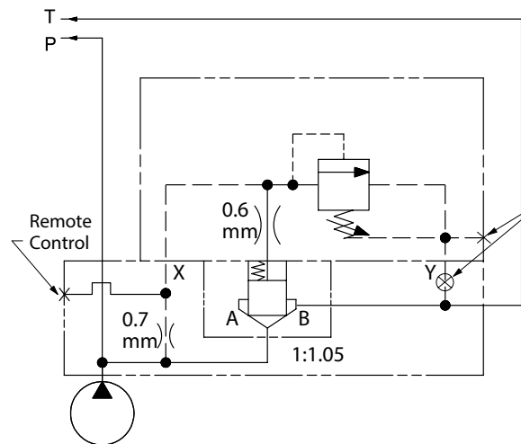
CPF1S-06/08-*-20 with remote control
