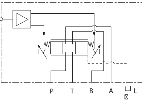
Model Type KBDG4V-5 Proportional directional valve (with integrated electronics)
