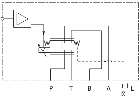
Model Type KBTG4V-5 Proportional throttle valve (with integrated electronics)
