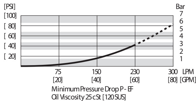
VLH P-EF Pressure Drop
