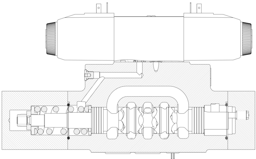
KDG5V-7 shown without "EX" or "X" (Without integral pilot pressure reducer)
