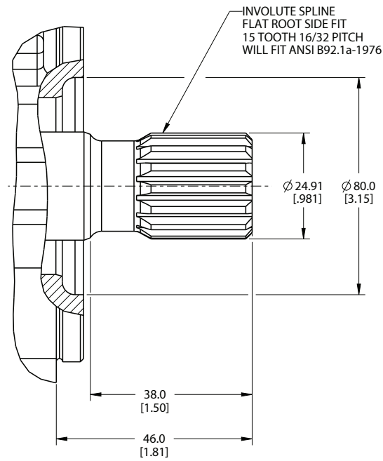
08 - SAE J744-25-4, SAE B-B, 15T SPLINE
