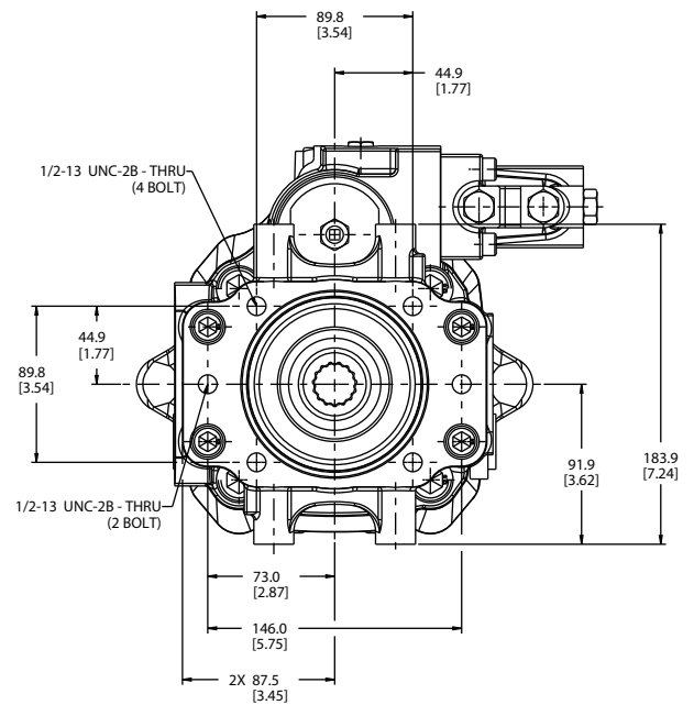
Right hand rotation Shown with Pressure Compensator with Load Sense
