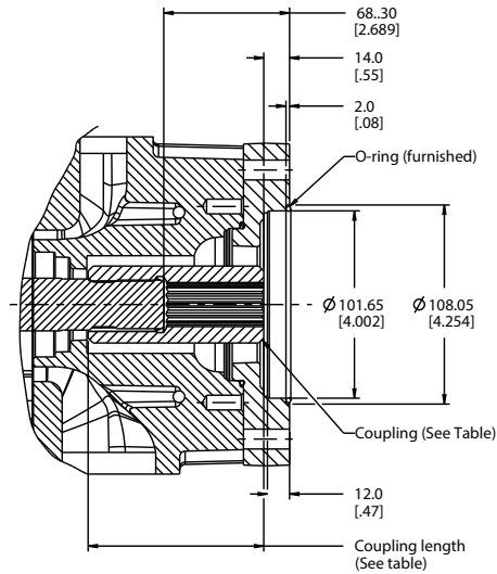
With adapter plate
