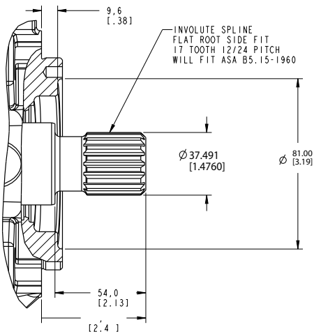
12 - SAE J744-38-4SAE "C-C" (17T)Spline
