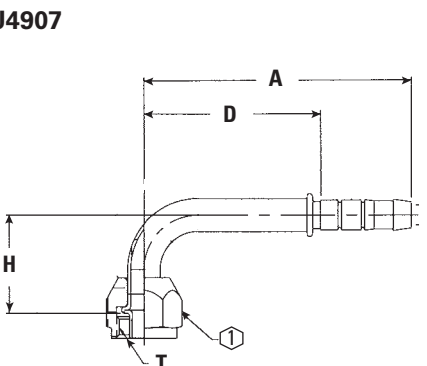
90° O-Ring (long pilot)
