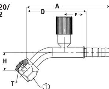
45° female O-Ring (short pilot) with charge port
