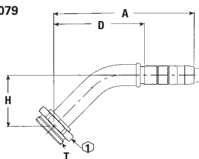
45° 5400 coupling thread
