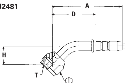
45° female O-Ring (long pilot)
