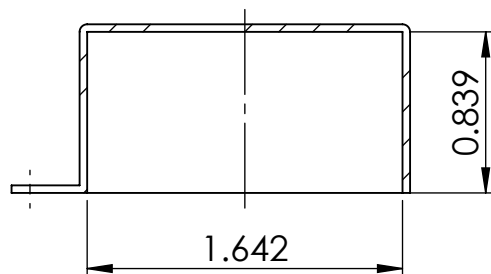
SECTION X-X
