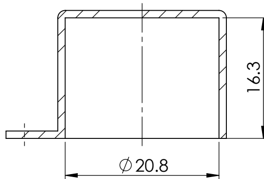
SECTION X-X
