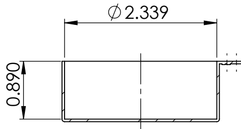
SECTION X-X
