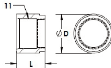
Half Couplings
