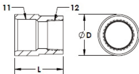
Full Couplings
