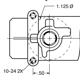
Mounting Detail
