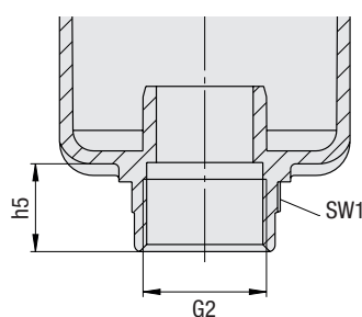
Threaded Outlet
