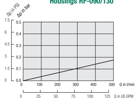
Housings RF-090/130
