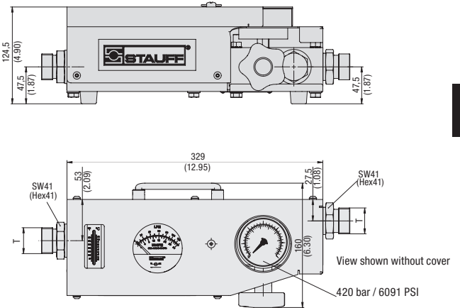
Dimensions SDMCR-750
